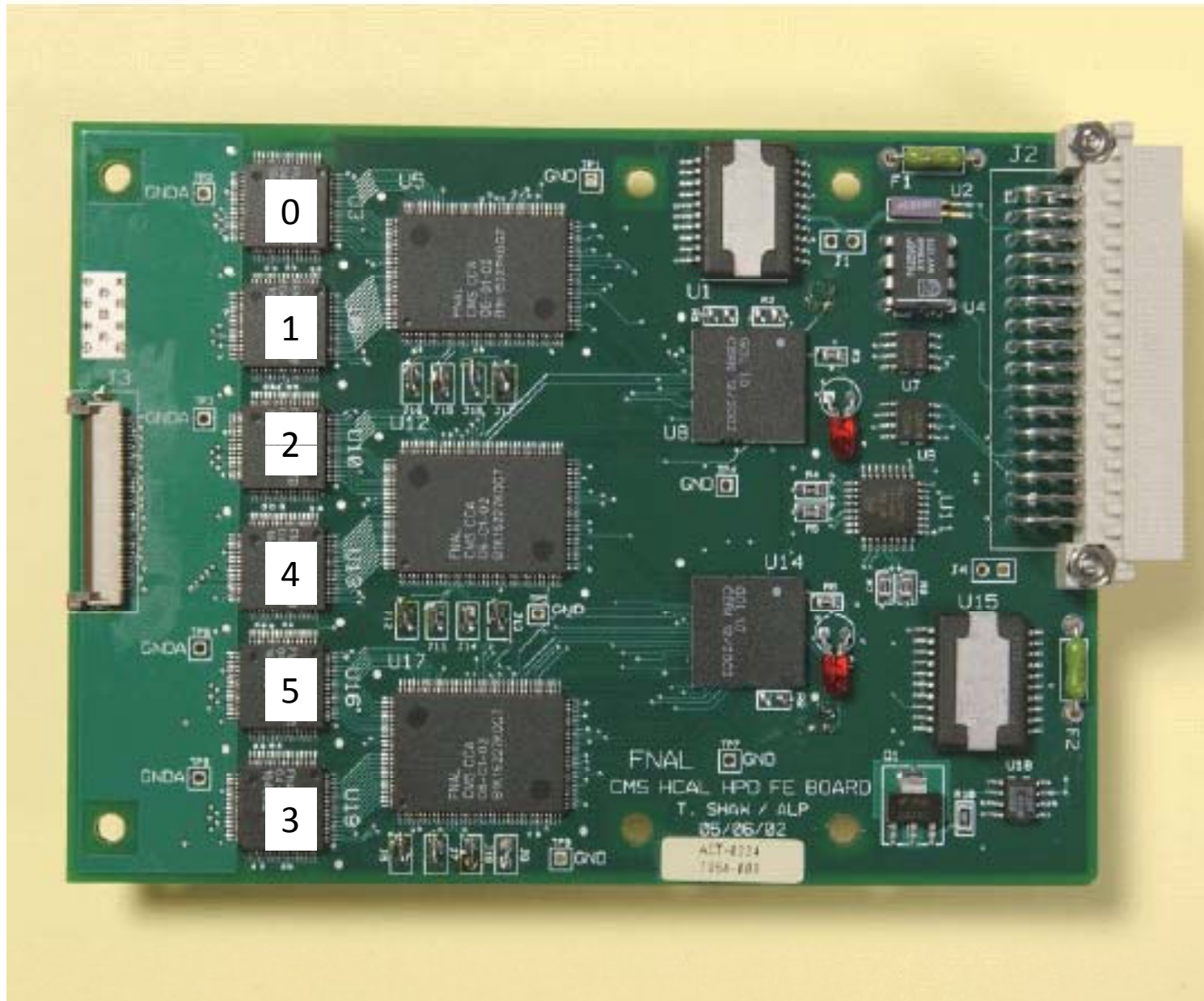
Figure 1. Photograph of the Testbeam 2002 Front End Module
