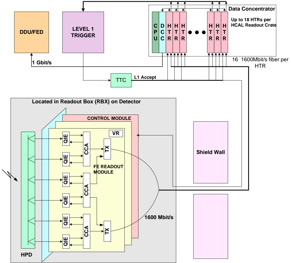
Figure 2. Readout System Overview
